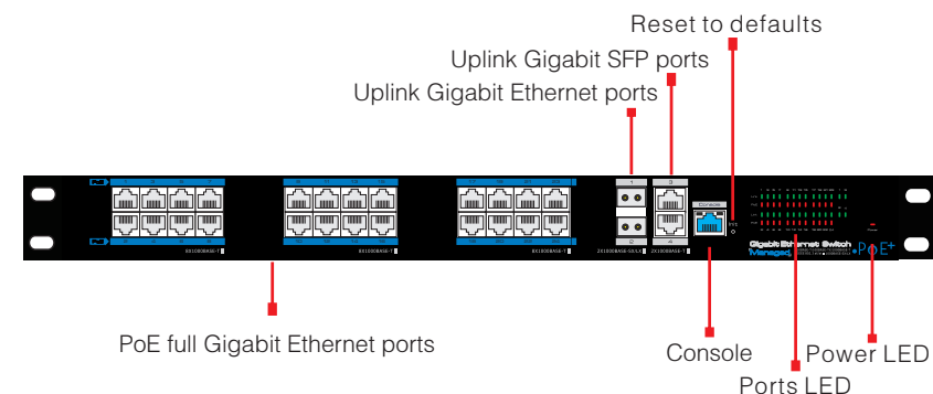
16 P Front panel
