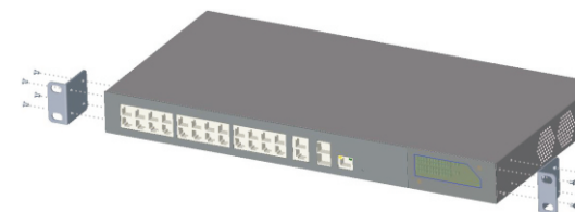
Figure 2-1 Install hangers diagram
